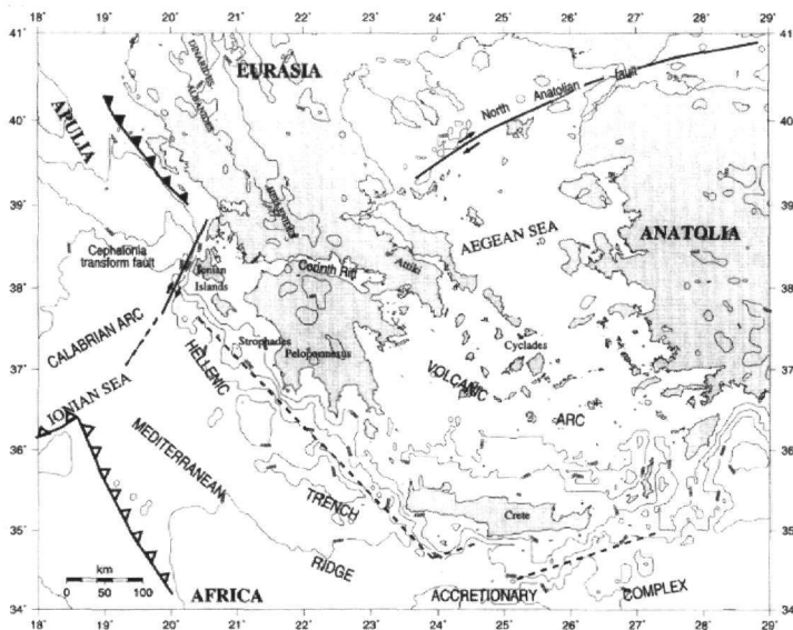
Figure 1 – Sketch map of the Ionian Islands of Western Greece in the Africa-Europe convergence region at the transition zone between Hellenic subduction in the south and continental collision in the north linked by the Cephallonia transform fault (Sachpazi et al. 2000)
