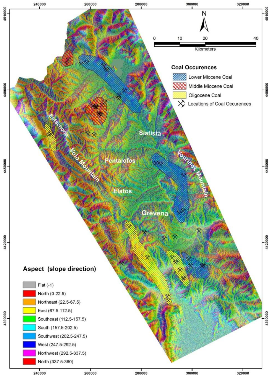
Fig. 3: Aspect function map of the Mesohellenic Basin with coal occurrences, based on Digital Elevation Modeling, displaying surface window of aspect algorithms and aspect directions.
