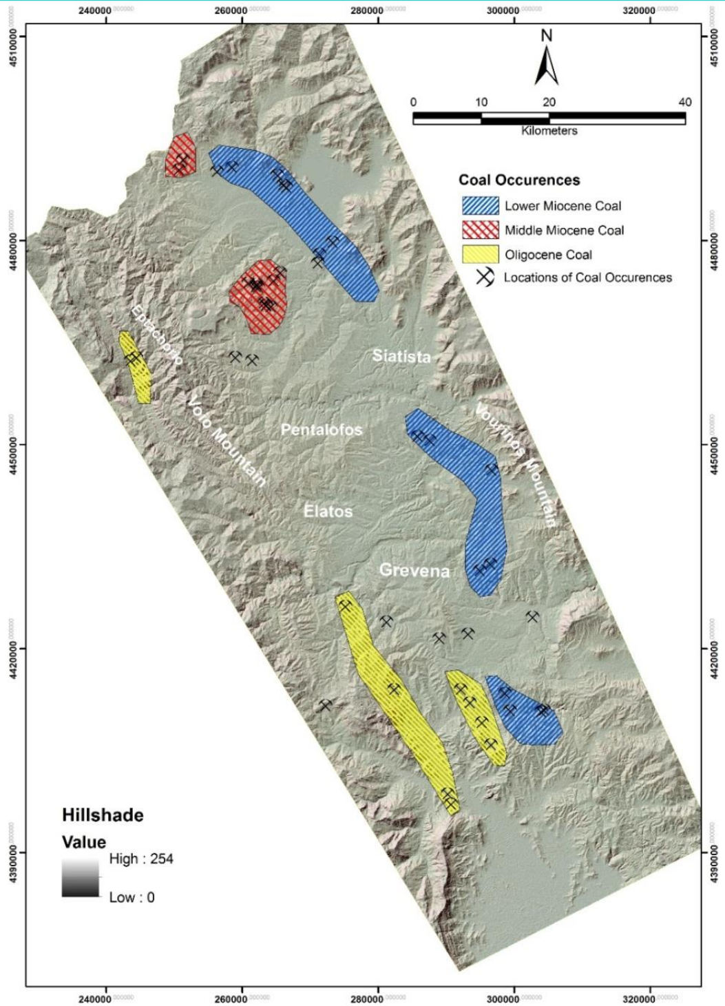
Fig. 5: Hillshaded Elevation Model of the Mesohellenic Basin with coal occurrences, based on Digital Elevation Model raster surface.
