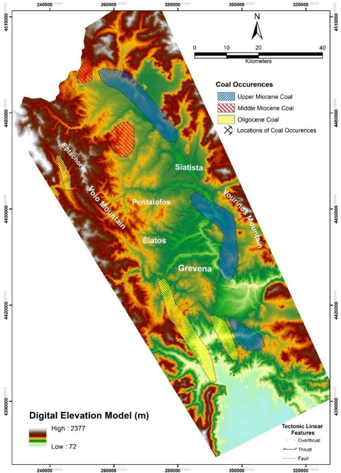
Fig. 2: Digital Elevation Model (DEM) map of the Mesohellenic Basin with Coal Occurrences (based on ASTER satellite dataset).
