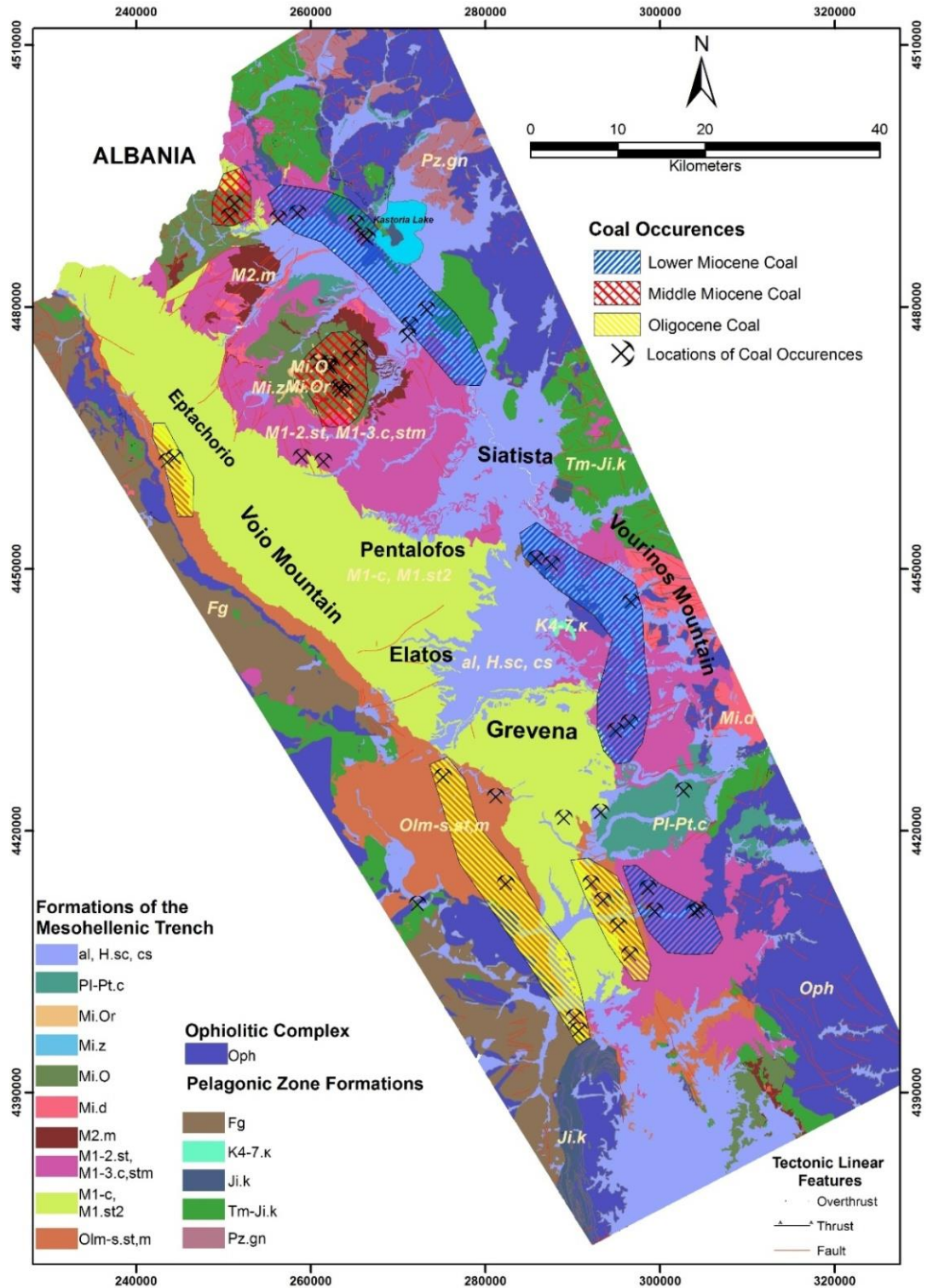
Fig. 1: Geological Map of the Mesohellenic Trough, indicating coal occurrences. Explanation of legend : al, H.sc, cs : Olocene deposits, Pl-Pt.c : Plio – Pleistocene conglomerate, Mi.Or: sandy marl, sandstone (Orlia
