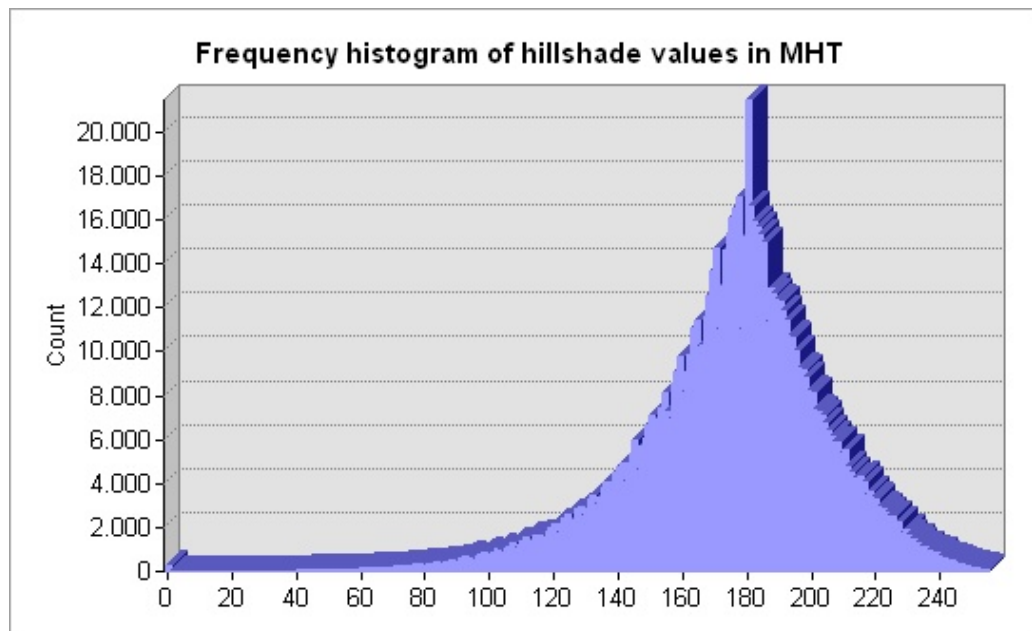
Fig. 6: Frequency histogram of hillshade values in MHT coal occurrences. The Y-axis (vertical axis) represents the frequency count of raster cells of each value, while the X-axis (horizontal axis) represents the values of each hillshade class.
