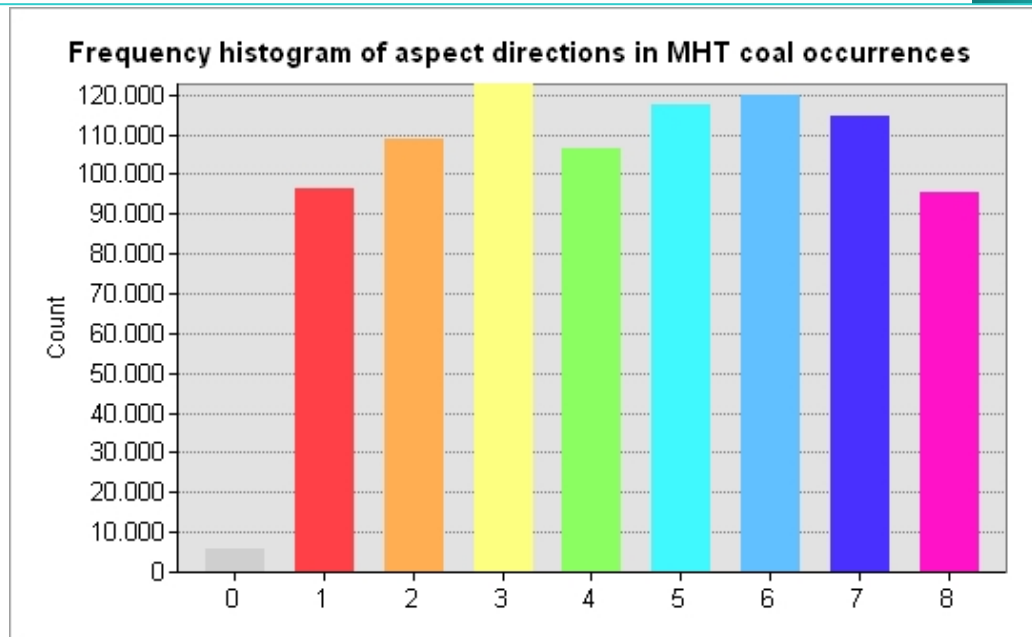
Fig. 4: Frequency histogram of aspect directions in MHT coal occurrences. Explanation of X axis values. (0 = flat, 1= North, 2 = Northeast, 3= East, 4 = Southeast, 5 = South, 6 = Southwest, 7 = West, 8 = Northwest). The Y-axis (vertical axis) represents the count of raster cells of each aspect class.
