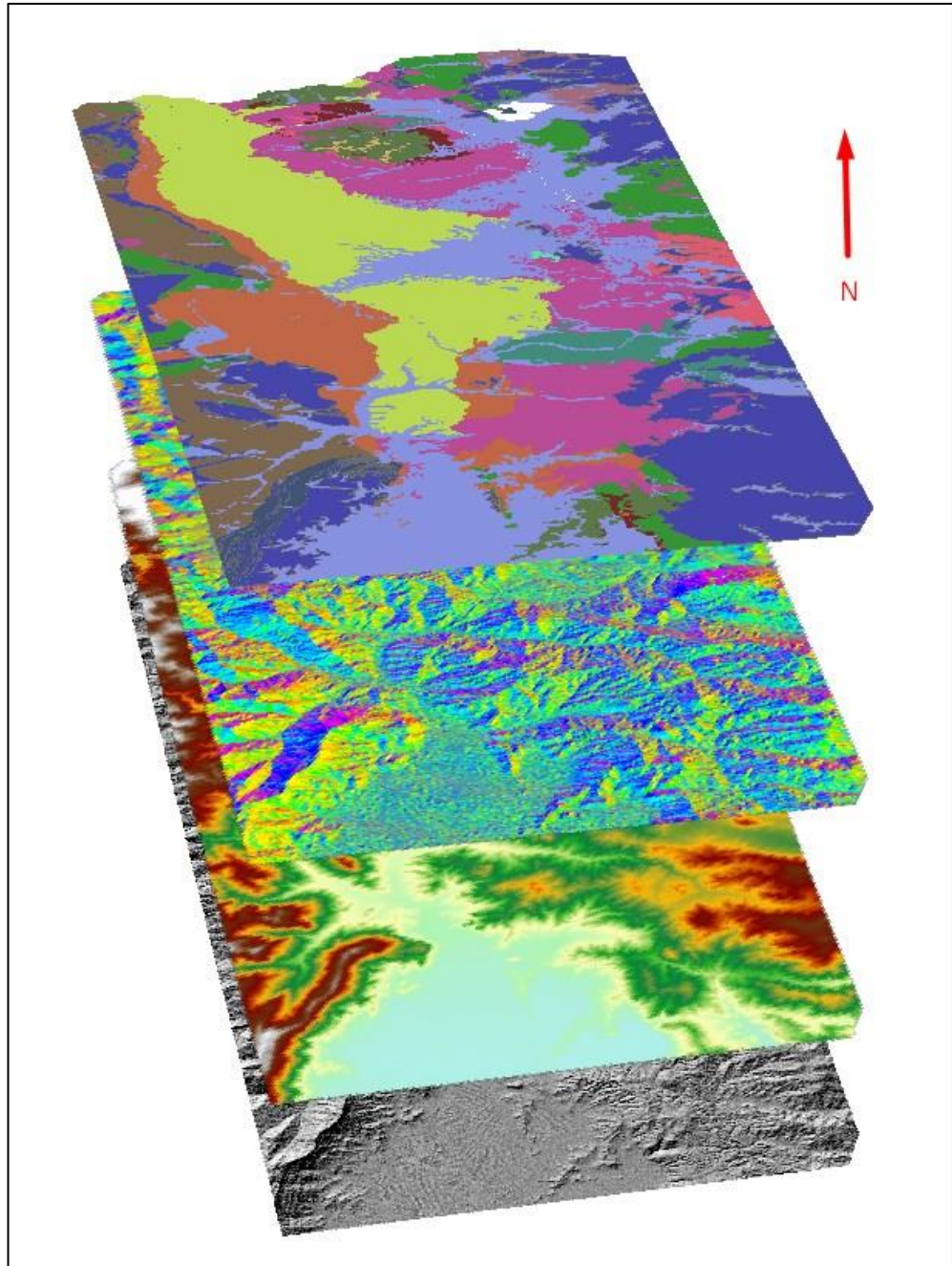
Fig. 7: 3D - overlay of thematic layers which used for zonal statistics and surface modeling related to coal occurrences in the Mesohellenic Basin.
