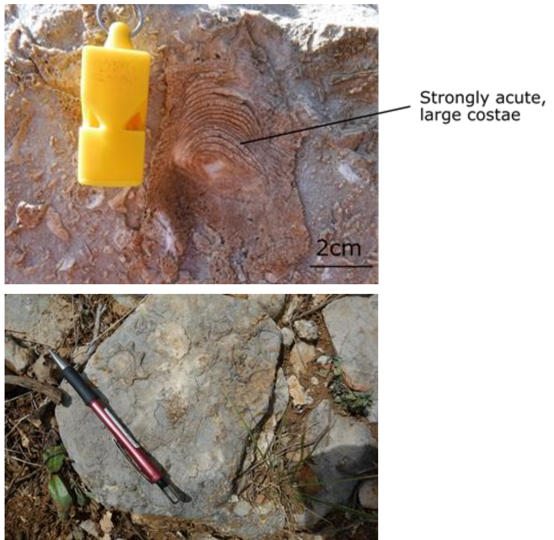
Fig. 10: top) transverse section through a Milovanovica, Radiolitidae which has undergone partial diagenetic alteration to ferroan dolomite. Bottom) cross-section of a star-shaped Milovanovica, Radiolitidae (Sari and Ozer 2009).
