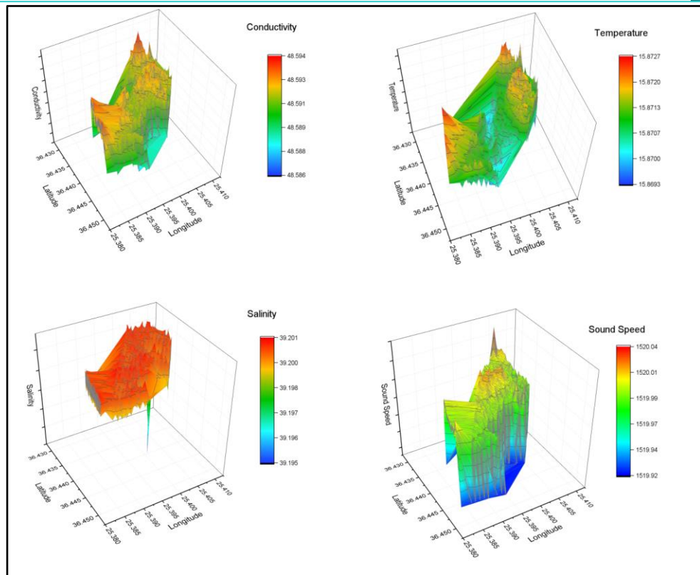
Fig. 5: Reconstructed 3D maps from recorded data of conductivity (S/m), temperature ( ^{\circ}\text{C} ), salinity ( \text{‰} ) and sound velocity (m/s), for the North-East area, investigated on the 11 th (Area A; dive #259). A high-resolution copy of this Figure can be found at the supplementary material.
