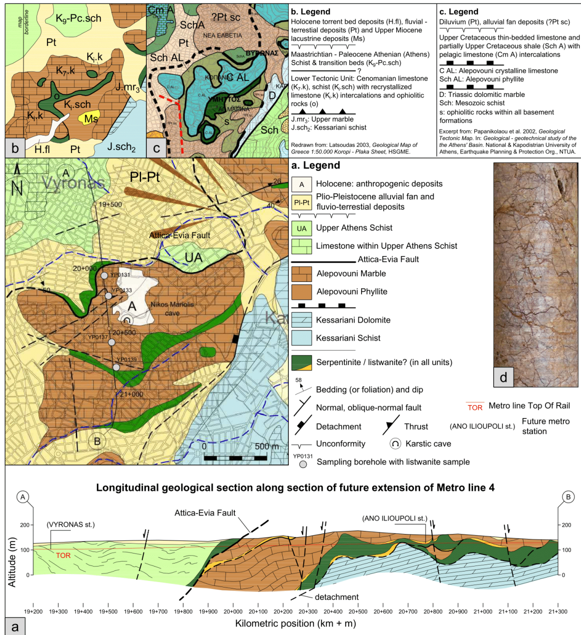
Fig. 9: a) Excerpt from the Geological Map of AMA at Vyronas and Ano Ilioupoli districts, based on “Geological map view - section ‘Evangelismos - Vyronas - Ilioupoli’ from K.P. 17+300 to K.P. 21+289” (dwg No 4G00PW180S102B), issued by “EDAFOMICHANIKI S.A. - ISTRIA GENERAL CONSULTANTS - ANESTIS PANAGOPOULOS” (2017). Longitudinal geological section A–B is based on “Geological and hydrogeological longitudinal section - section ‘Evangelismos - Vyronas - Ilioupoli’ from K.P. 17+300 to K.P. 21+289” (dwg No 4G00PW180S403B), issued by “EDAFOMICHANIKI S.A. - ISTRIA GENERAL CONSULTANTS - ANESTIS PANAGOPOULOS” (2017) (b) and (c) show the excerpts from HSGME and Papanikolaou et al. (2002) geological maps respectively, of the same area, for comparison. Scale of (b) and (c) maps is half the scale of (a) map d) Core of pink, fractured, massive, fine grained marble, Alepovouni Marble, Vyronas district.
