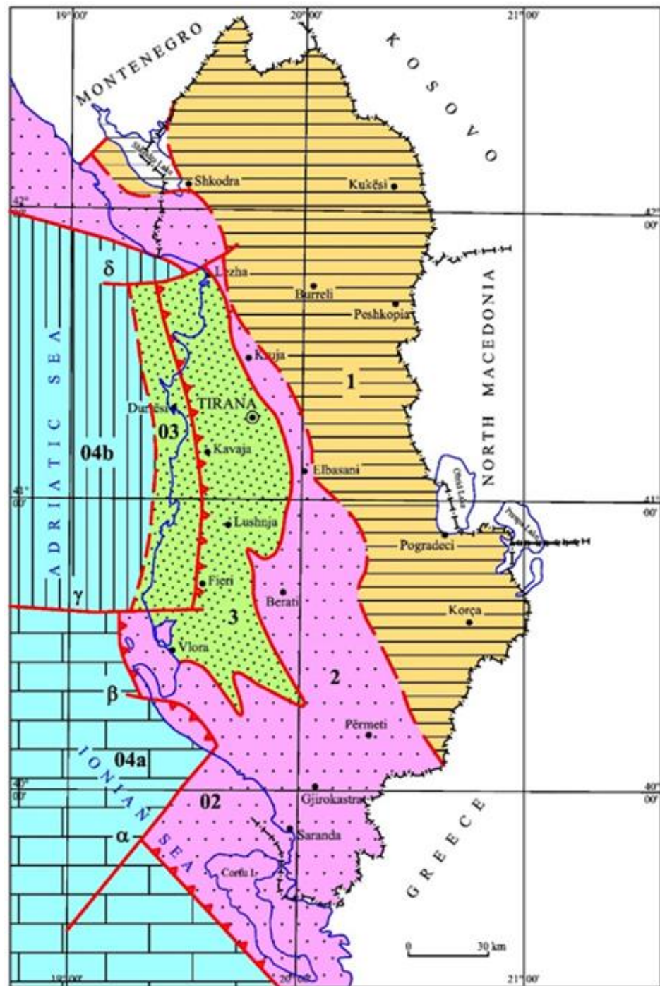
Fig. 4: Map of the neotectonic (Pliocene-Quaternary) zonation of Albania (and Corfu Island of Greece) shows the large neotectonic units of Albania (after Aliaj et al., 1995, published in 2018 ). The orogen front from south to north is cut and displaced by the Othoni Island-Dhermi ( \alpha ), the Gjiri i Ariut-Dukat ( \beta ), the north of Sazani Island ( \gamma ), and the Gjiri i Drinit-Lezha ( \delta ) transversals. The large neotectonic units of Albania shown by numbers are the following: 1: The internal area affected by extensional tectonics since Pliocene, 2: the external area affected by compressional pre-Pliocene tectonics, 3: the Peri-Adriatic Foredeep strongly affected by post-Pliocene compressional tectonics (03: its offshore sectors), 04: Pliocene-Quaternary Foreland in Adriatic and Ionian offshore (04a: Apulian platform. 04b: Albanian Basin).
