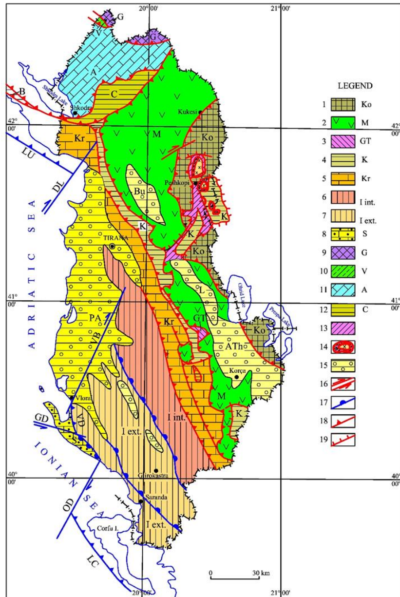
Fig. 2: Tectonic Map of Albania shows the Drini Bay-Lezha (DL) and Vlorë-Bishqumi (VB) strike-slip faults in blue colour that led to the development of the Periadriatic Foredeep (PA) as well as the active Albanides collision zone thrust faults (modified from Aliaj, 2021). OD- Dhermi-Othoni Island dextral strike-slip fault that separates the Albanides – Hellenides segments: VD- Vlorë-Dhermi segment from LC- Lefkas-Corfu one. LU-Lezha-Ulqini segment belongs to the Dinarides. The GD- Gjiri i Ariut - Dukat i Ri and OD -Othoni Island-Dhermi strike-slip faults bound the Sazani Zone Mali i Kanalit Block that backthrusts towards NNE the Ionian Zone Çika anticlinal belt. Tectonostratigraphic units: 1- Korabi, 2- Mirdita, 3- Guri i Topit, 4- Krasta, 5- Kruja, 6- Internal Ionian, 7- External Ionian, 8- Sazani, 9- Gashi, 10- Vermoshi, 12- Cukali. 13- Upper Jurassic-Lower Cretaceous marly flysch underlying Korabi nappes, 14- Kruja zone evaporite dome surrounded by the Upper Eocene-Lower Oligocene flysch. 15- Molasses basins: ATh-Albanian-Thessalian, L-Librazhdi, Bu-Burreli, and PA- Periadriatic basins. 16- Dextral and sinistral strike-slip faults, 17-Reverse fault, 18- Thrust, 19-Normal fault.
