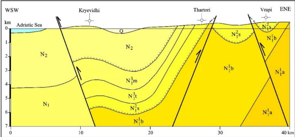
Fig.16: The Kryevidhi-Vrapi geological section shows the Periadritic Depression structure with its deepest Myzeqe depocenter of the Middle Miocene-Pliocene molasses that is located to the west of the Thartori-Mliku high.
