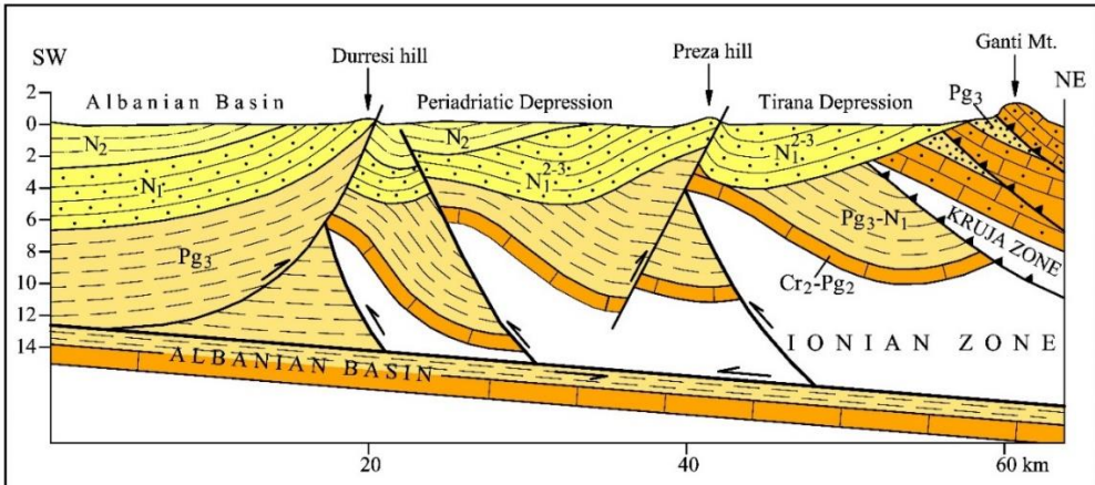
Fig. 17: Geological cross-section through the Duresi hill-Preza hill-Ganti Mt. showing the collision between the Albanian Basin and the Ionian Zone blind thrust-bounded imbricates which are unconformably overlain by the Middle Miocene-Pliocene molasse of Periadriatic and Tirana depressions (after Aliaj, 2020).
