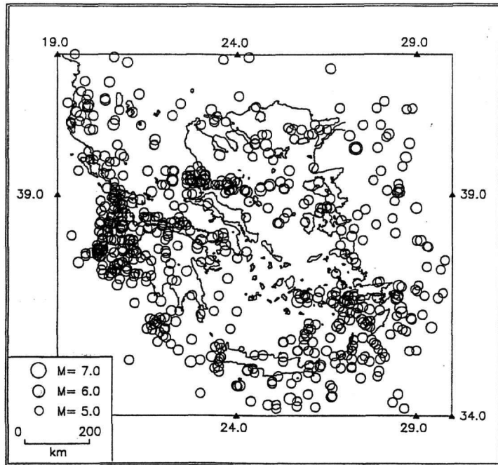
Figure 2. Spatial distribution of 632 located earthquakes during the period 1950 – 2000 and having M_l > 5.0 .
