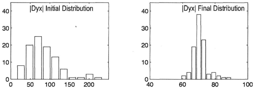
Figure 2. Left: The distribution of the original \{D_n\} population illustrated in Figure 1. Right: The final distribution of the processed ensemble, after application of the robust W-estimator (see Figure 3).
