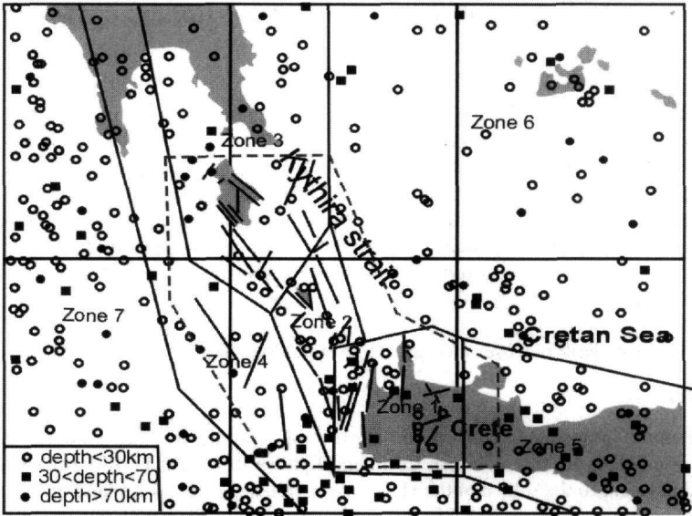
Angelier et al., 1992), the area sources, and the polygon for which, hazard is calculated.
