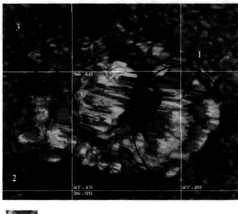
Figure 3. Differential Interferogram image (ERS-2, 11-6-96/6-7-99) of Nisyros Island (Magnitude & Phase). One fringe is visualized as a cycle of gray levels intensities.
