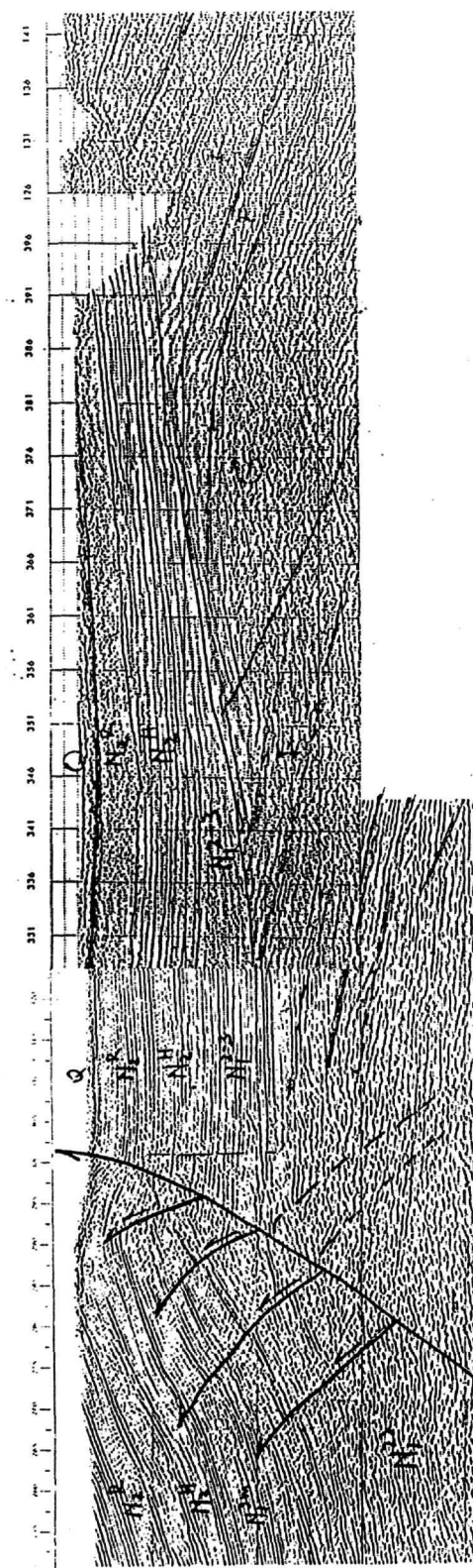
Fig. 5 - Seismic line in Ardenica - Marinza region The "flower" type structure faults of "palm tree" type in Ardenica anticline, the unconformity between Miocene molasses and underlying folded flyschs and carbonatic deposits of Ionian zone and the slight unconformity between the Pliocene molasse and the Miocene molasses are shown.
