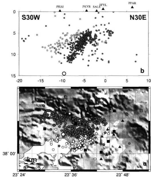
Figure 3. Aftershocks (grey circles) and main event (large open circle) of the 1999/9/7 event. Squares denote stations of the aftershock network, while triangles denote strong motion instruments.
