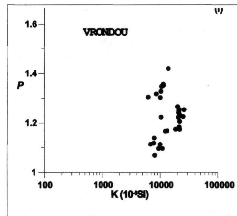
Figure 3: Anisotropy degree ( P ) versus magnetic susceptibility ( K ) plot. Roughly, according to Rochette (1987) the upper limits of the paramagnetic contribution are K > 300-500 \cdot 10^{-6}SI and P > 1.2 .
