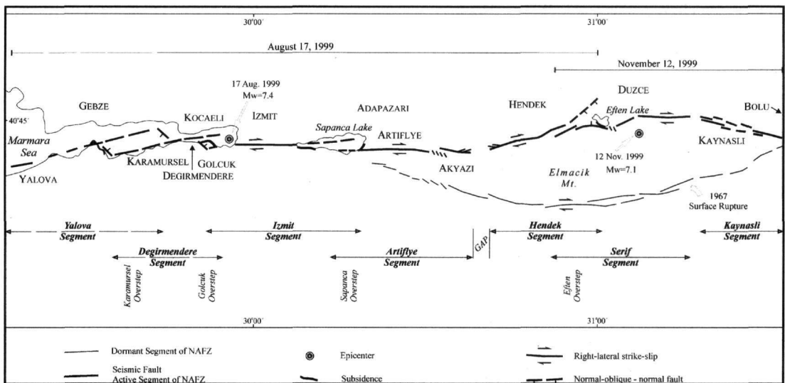
Fig. 2 The traces of the segments reactivated in the 17 August and 12 November 1999 earthquakes. and associated structures. Finally, a comparison between our observations and the results of previous studies will be attempted.
