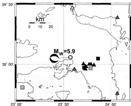
Figure 1. Epicenter of the Athens 1999/9/7, M_w=5.9 mainshock. Squares denote stations with P_g or S_g arrivals, while triangles denote stations with P_g-S_g traveltimes.
