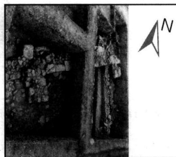
Figure 6. Excavation that show the unearthed foundations of an inner wall. This structure, along with its fallen towards north upper structure produced the linear anomaly observed in the Southwest of the surveyed area.
