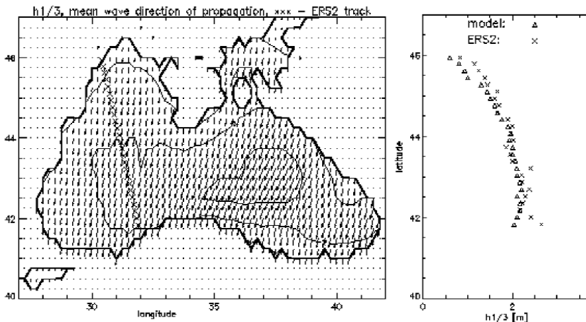
Fig. 1: The VAGBUL1 model output along with the satellite ERS-2 values of SWH for 29th December at 20:00.
