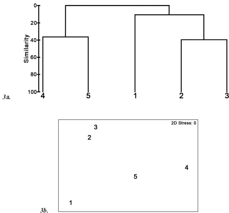
Fig. 3: Grouping of stations based on macrozoobenthos composition produced with a) Bray-Curtis group average clustering technique and b) MDS ordination.
