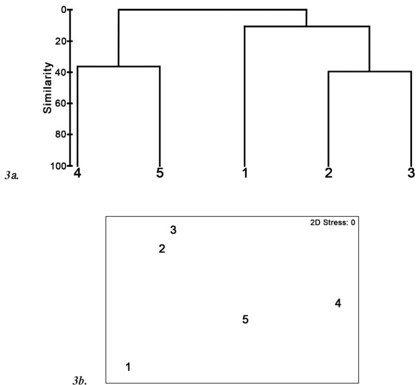
Fig. 3: Grouping of stations based on macrozoobenthos composition produced with a) Bray-Curtis group average clustering technique and b) MDS ordination.
