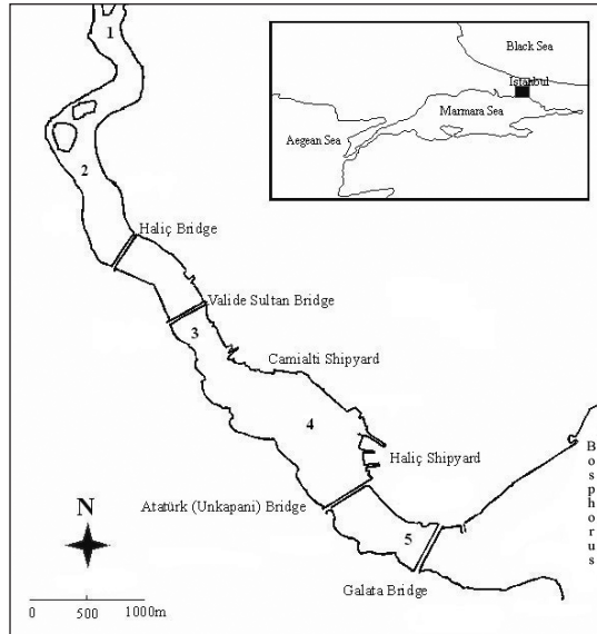
Fig. 1: Map of Golden Horn Estuary showing location of sampling stations.
