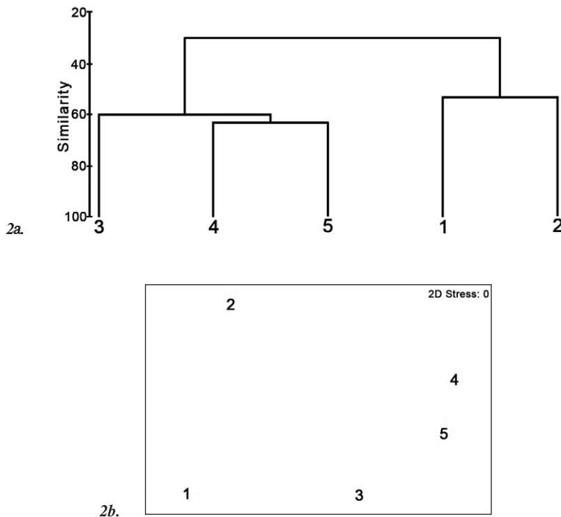
Fig. 2: Grouping of stations according to phytoplankton composition produced with a) Bray-Curtis group average clustering technique and b) MDS ordination.
