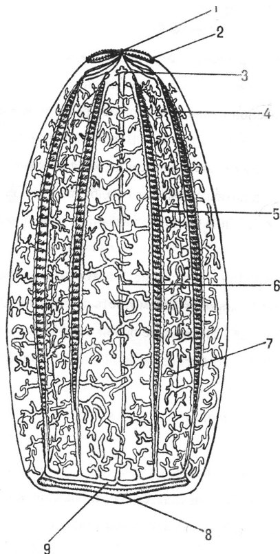
Fig. 2: Morphology of Beroe cucumis (after Mayer, 1912) 1- aboral organ; 2- polar plate; 3- ifundibulum; 4- subsagittal comb row; 5- subtentacular comb row; 6- paragastral canal; 7- diverticuli; 8- mouth; 9- labial canal.
