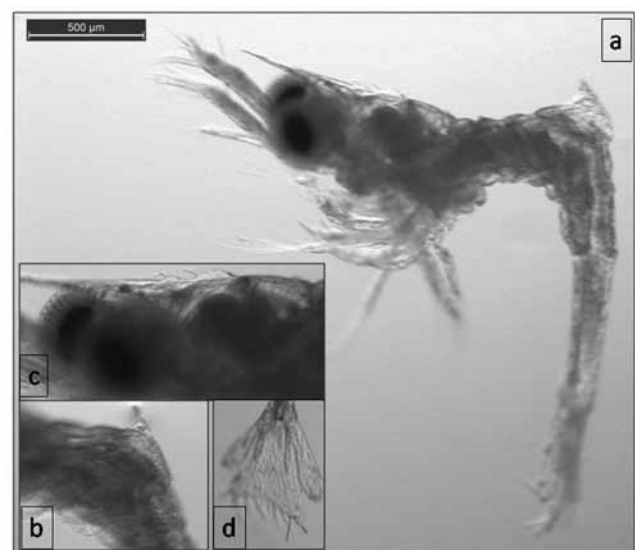
Fig. 3: Palaemon macrodactylus , Zoea III captured in the Balearic Sea in 2010, general view (a) whole lateral view, (b) abdominal dorsal spine detail, (c) rostral dorsal spines and (d) telson.
