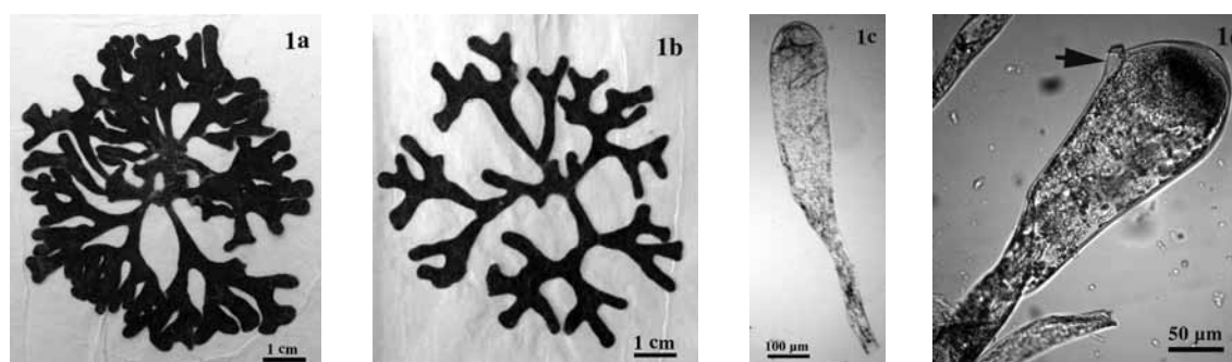
Fig. 1: Codium taylorii : (a) general view of thallus (December 2011); (b) habit with cervicorn terminal ramification (October 2011); (c) utricle; (d) utricle with hair scar (arrow).
