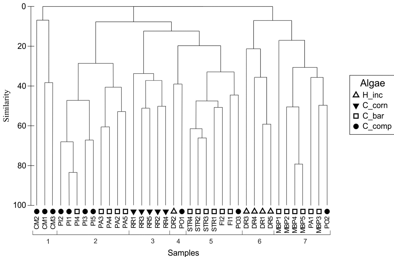
Fig. 5: Cluster of samples associated with four canopy-forming algal species ( H_inc = H. incurva ; C_corn = C. corniculata ; C_bar = C. barbata ; C_comp = C. compressa ), based on mollusc abundance data. Groups were formed with a cut at 20% of similarity.
