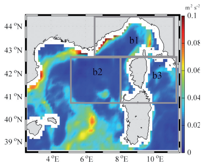
Fig. 3: Mean Absolute Difference of Kinetic Energy based on AVISO and ROMS_NWMed data.
