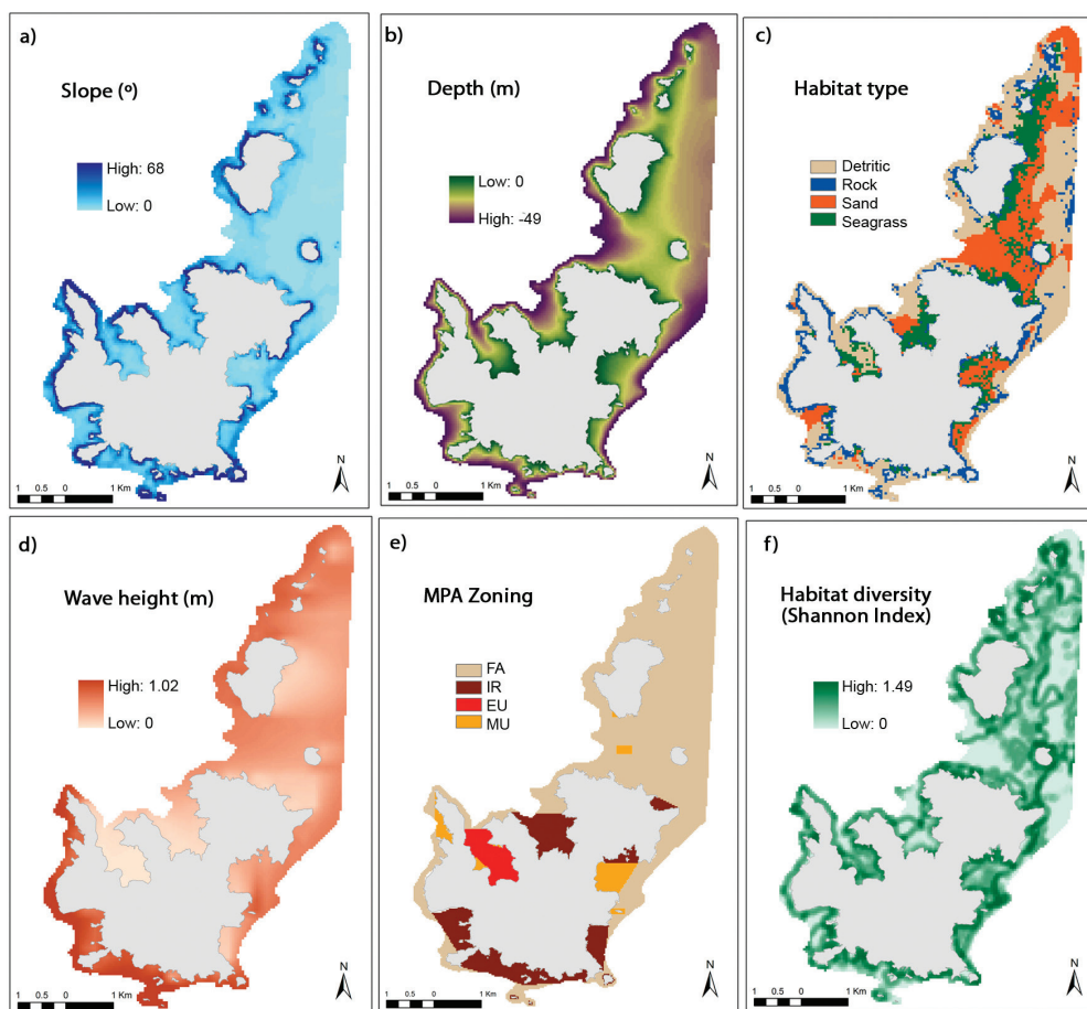
Fig. 2: Environmental variables used to model P. nobilis densities. a) Slope, b) Depth, c) Habitat type, d) Wave height ( H_s ), e) MPA zoning: FA, fishery allowed; IR, integral reserve; EU, especial use; MU, moderate use; and f) Habitat diversity (Shannon Index).
