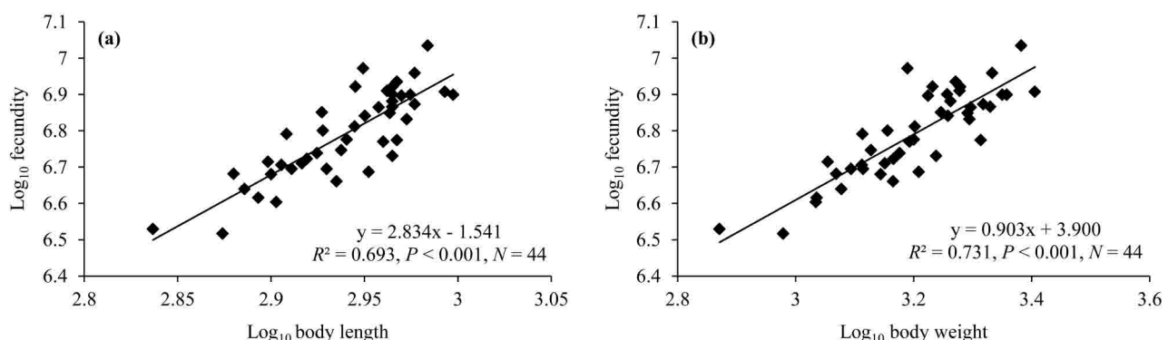
Fig. 3: (a) \text{Log}_{10} -transformed fecundity–body length and (b) fecundity–body weight relationships.
