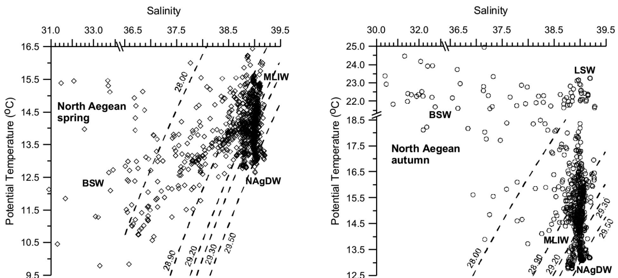
Fig. 3: \theta -S diagram in the North Aegean Sea (all data were used) during spring and autumn for the 1987-2008 period.
