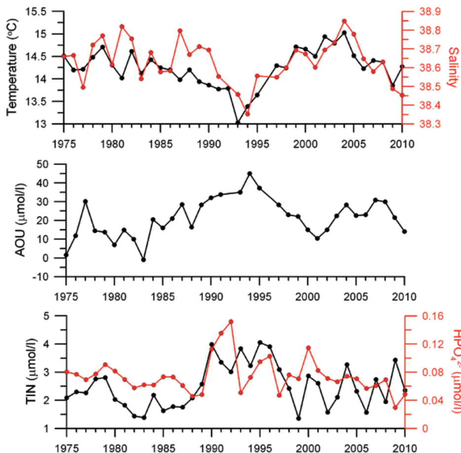
Fig. 4: Annual time series of temperature, salinity, apparent oxygen utilisation (AOU), total inorganic nitrogen (TIN) and ortho-phosphates ( \text{HPO}_4^{2-} ), all collected at station S between 1975 and 2010.
