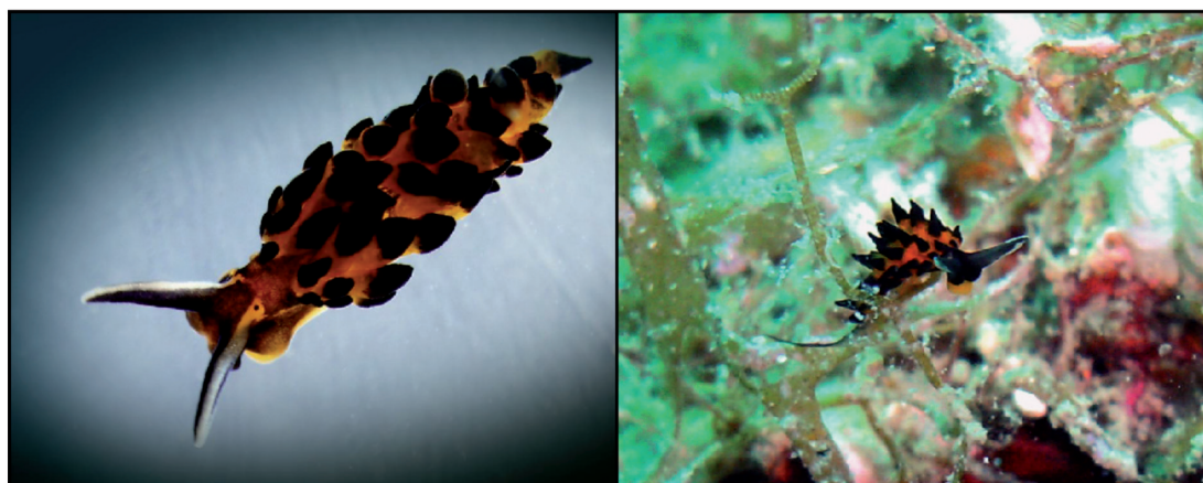
Fig. 5: Specimens of Placida cremoniana found in Slovenian waters. Left: a specimen found on a carpet of Corallina sp. (Photo: B. Mavrič), Right: specimen grazing on filamentous algae at Fiesa (Photo: G. Zadnik).
