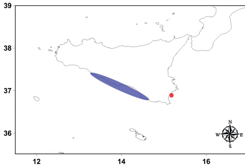
Fig.10: The semi-transparent blue zone indicates area of the past record of O. cursors in Sicily; the red dot indicates the first and new records of the species in the Ionian Sea (Avola).
