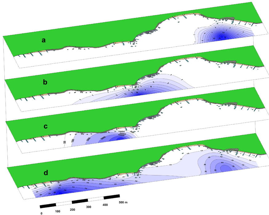
Fig. 2 a-d: Study area (60 sites, solid yellow line) and area of recording (dotted brown line) of the alien mollusc A. kagoshimensis along the CSpatial variability of the biomass distribution ( \text{g/m}^2 ) of the alien molluscs, A. kagoshimensis (a) and R. venosa (b), of the alien crab R. harrisi (c), and of the all macrozoobenthos (d) at one of the investigated sites (“2” on the map, Fig. 1).
