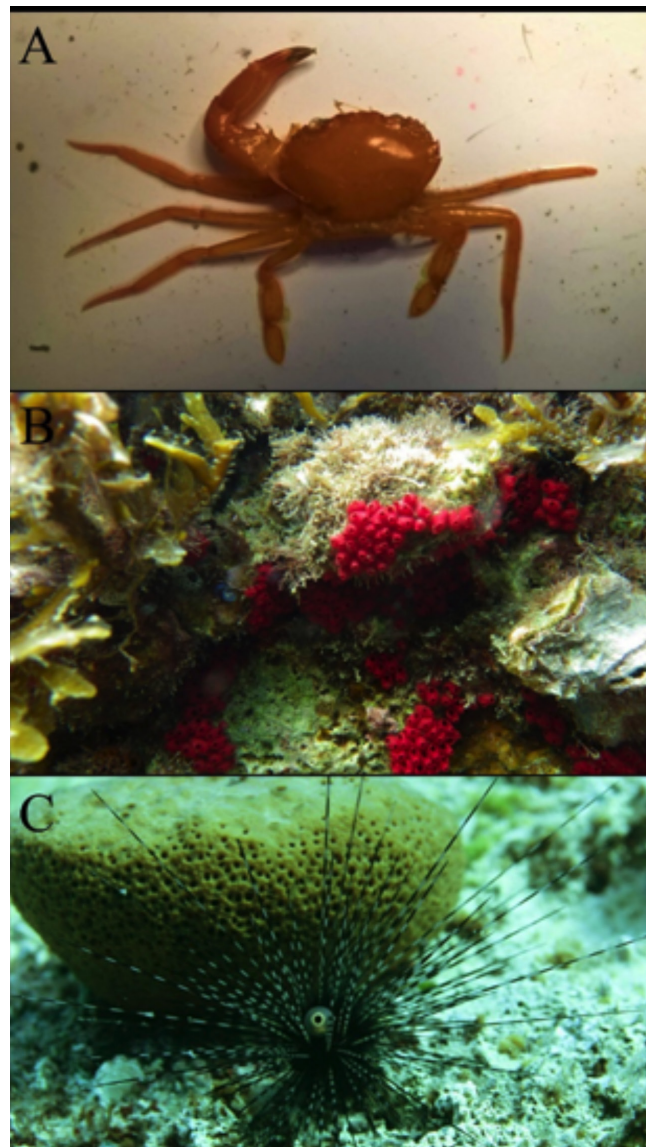
Fig. 22: A–C. New alien species reported from Cyprus. A. The crab Carupa tenuipes (Dana, 1852). B. The ascidian Symplegma brakenhielmi (Michaelsen, 1904). C. The sea urchin Diadema setosum (Leske, 1778).
