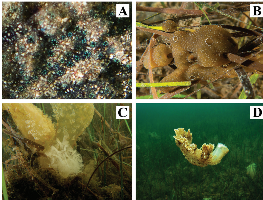
Fig. 15: A) Close up of the colonial ascidian Aplidium coeruleum . In each siphone, six blue lobes are distinguished, diagnostic character of the species. B) The colonial ascidian Didemnum protectum surrounding leaves of Cymodocea nodosa . C) Spawning of an individual of the alien nudibranch M. viridis in a Cymodocea nodosa meadow. D) M. viridis in the inner part of Messolonghi lagoon, many individuals are distinguished in the background. (Photos A-C: by Christos Kotselis, D: by Eleni Kytinou).
