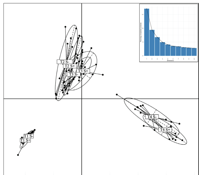
Fig. 5: Result of PCA run on frequency data of the fouling species at four sampling times (T1, T2, T3, T4) for controls (with Sabella spallanzanii = S+) and treatments (without Sabella spallanzanii = S-). The first two PC axes explain the 17.05% and 9.392% of the total variance, respectively. The explained variance of the first 10 axes are reported in the histogram box.
