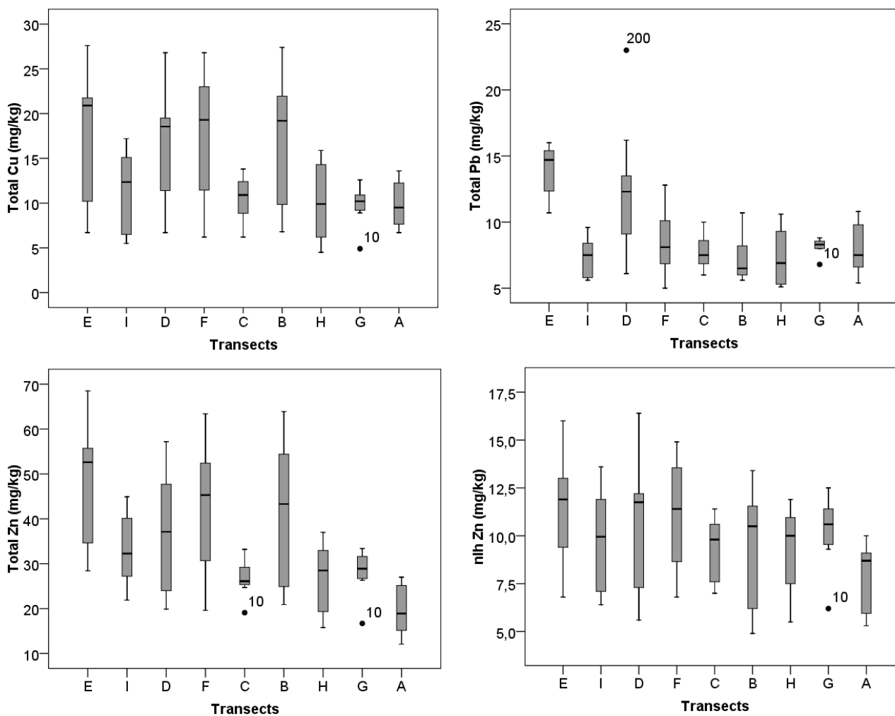
Fig. A5: Total Cu, Pb and Zn and nlhZn per transect [transects are presented from west to east, (•) the outlier value symbol and numbers refer to the isobaths].
