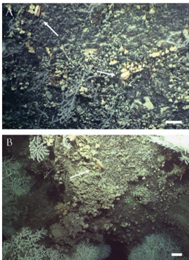
Fig. 3: Acesta excavata (pointed by white arrows) on vertical canyon walls surrounded by Desmophyllum dianthus , Murielidae lepida (A), and by Desmophyllum pertusum and Madrepora oculata (B). Scales are 10 cm apart in both images.
