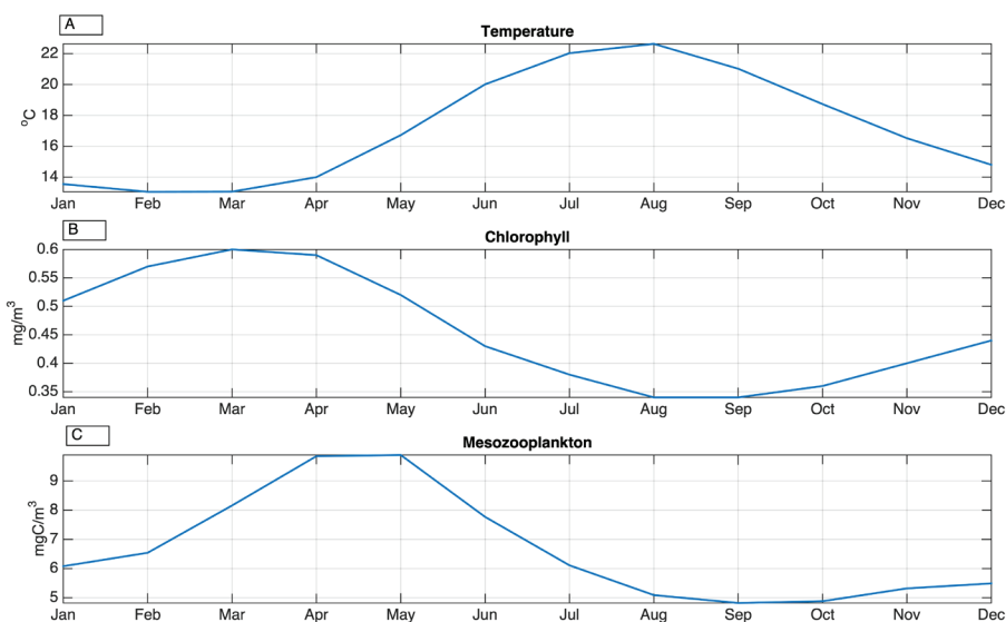
Fig. 4: Mean (2000-2009) seasonal evolution of A) simulated sea surface temperature ( ^{\circ}\text{C} ), B) chlorophyll ( \text{mg}/\text{m}^3 ) and C) meso-zooplankton biomass ( \text{mgC}/\text{m}^3 ).
