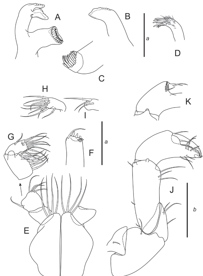
Fig. 20: Leptocheilia tanykeraia non-ovigerous female. A, left mandible; B, right mandible incisor; C, right mandible molar; D, maxillule endite, distal; E, maxilliped bases, right palp articles 2-4, left palp articles 3-4, and endites omitted for clarity; F, maxilliped endite; G, maxilliped palp articles 3-4; H, maxilliped palp article-4; I, maxilliped article-4 obscured setae; J, right cheliped; K, left chela, mesial view. Scale lines: a, 0.125 mm, A-I; b, 0.25 mm, J-K.
