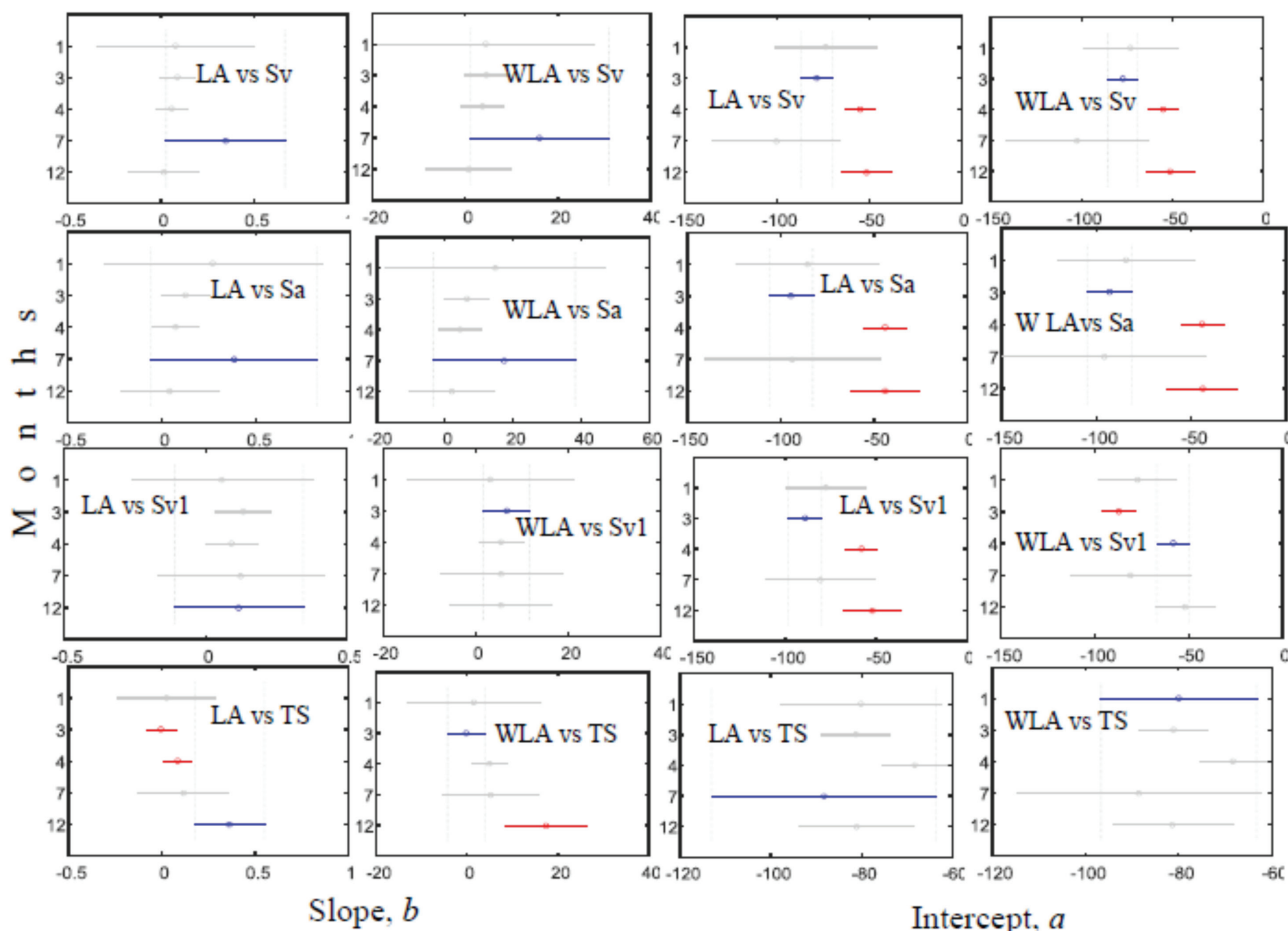
Fig. II: The post hoc test (Least Significant Difference, LSD) of seasonal relationship based on regression coefficients between acoustic data of Sv, Sa, Sv1, and TS, biometric variables (LA and WLA) with leaf + base of P. oceanica (blue mark: to be tested among the months or depths, red: significantly different, grey: significantly not different between vertical discrete grey lines) (see Appendix 1 for the abbreviations).
