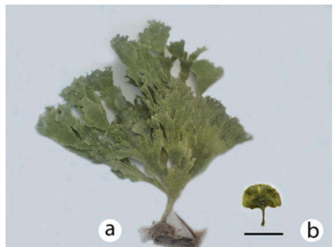
Fig. 3: Difference between a) Udotea flabellum and native Mediterranean species b) Udotea petiolata (the scale length is 4 cm).
