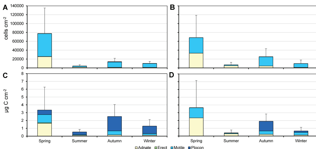
Fig. 4: Abundance (cells cm -2 , A, B) and biomass (μg C cm -2 , C, D) of epipellic diatoms at Portonovo (A, C) and Senigallia (B, D) stations in the different seasons, with the contribution of each growth form. Bars indicate standard deviation (of the total).
