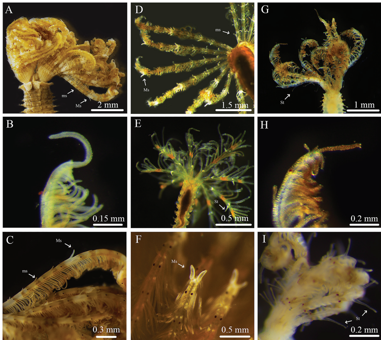
Fig. S25: Comparison of radiolar tip and stylodes among Branchiomma K lliker, 1858 material analysed in this study. A-C. Branchiomma boholense (Grube, 1850) from Lebanon coasts (A. Anterior end and crown, fixed material; B Radiolar tip, fixed material; C. Close-up to macro- and micro-stylodes, fixed material); D-F. Branchiomma boholense (Grube, 1850) from Italian coasts (D. Medium size alive specimen, with macro- and micro-stylodes distinct; E. Small size alive specimen with stylodes in development; F. Close-up to macro-stylodes, frontal view); G-I. Branchiomma bairdi (McIntosh, 1885) from Lebanon coasts (G. Anterior end and crown, fixed material; H. Radiolar tip, fixed material; I. Close-up to stylodes, fixed material). Ms. macro-stylodes; ms. micro-stylodes; st. stylodes.
