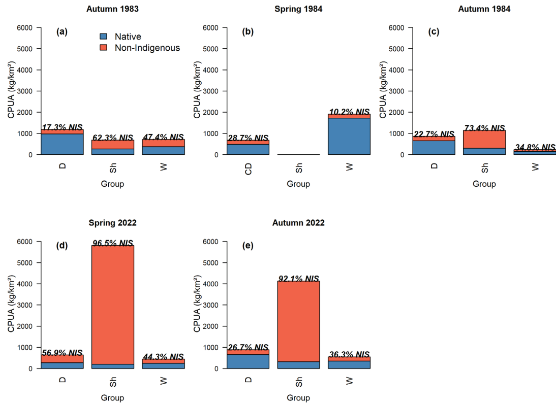
Fig. A2: Total CUPA (kg/km²) of sampling periods per cluster, partitioned into native and non-indigenous species (NIS) based on their proportional contributions (%). Years are indicated above each panel; bar height represents total CUPA, and segments show the relative contributions of native and NIS species within each cluster.
