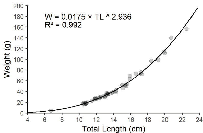
Fig. S1: Length-weight relationship for Morocco dentex individuals caught in the central Adriatic Sea (N = 47).
