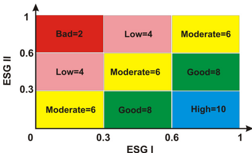
Fig. 2: Estimation of EECI and the equivalent EECs from a matrix based on the mean abundance (%) of ESGs.
