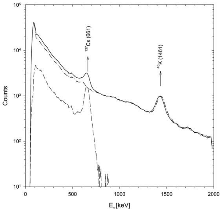
Fig. 2: Gamma ray spectrum recorded in the laboratory (3 days) by mixing in drinking water KCl (dashed double dot line), and adding known activity concentration of ^{137}Cs (solid line). The dashed line represents the pure ^{137}Cs spectrum deduced by subtracting the previous two spectra.
