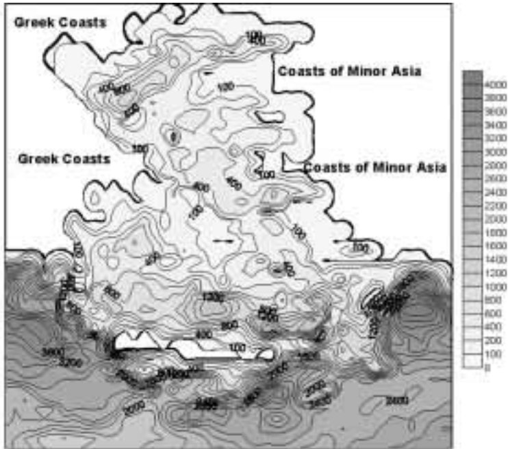
Fig. 7b: Thickness of the lower layer under the influence of the Etesians for 6 days (thickness in m).
