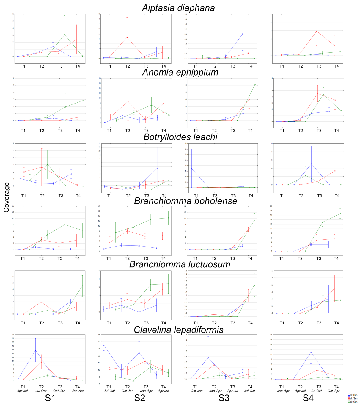
Fig. S1: Variability of coverage for species from BVSTEP (bars represent standard error) during the community development in each panel set (S).
