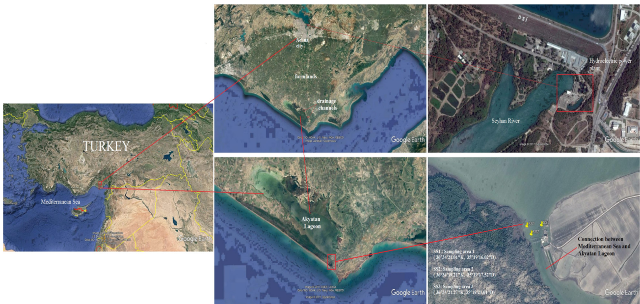
Fig. 1: Location of the sampling area of Akyatan Lagoon and its drainage channel to Mediterranean (Google Earth Inc. 2017).
