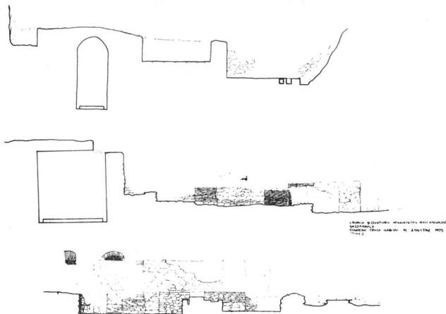
Σχ. 9. Ἡ Τομὴ τοῦ λουτροῦ τῆς ὁδοῦ Μαβίλη 9.
