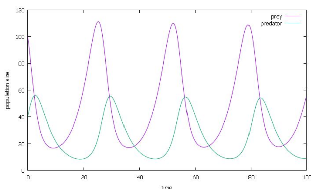
Figure 6.2: Lotka-Volterra model with b = 0.04
