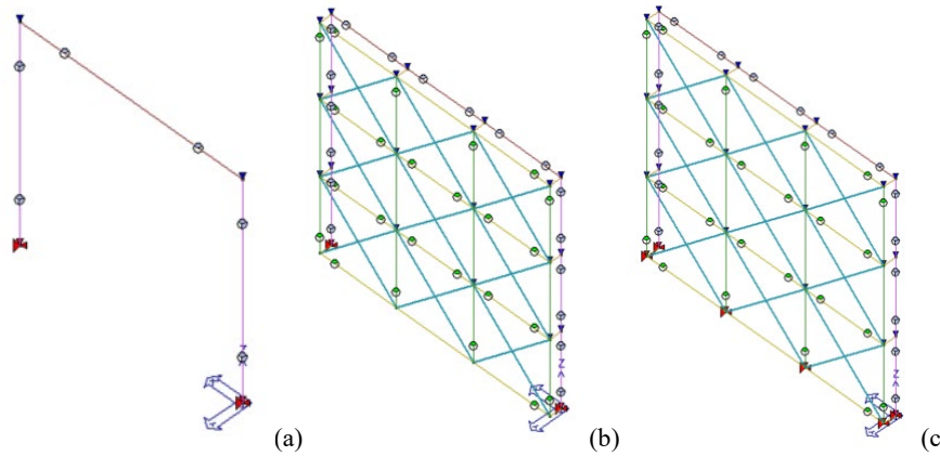
Fig. 18. Wireframe graphic of the three models: RC Frame (a), RC Frame + Resisto NOT Fixed in foundation (b) and RC Frame + Resisto Fixed in foundation (c).
