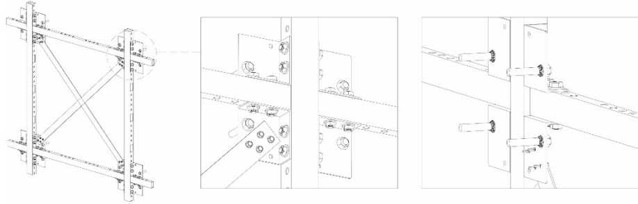
Fig. 9. Components of the Resisto 5.9 system.
