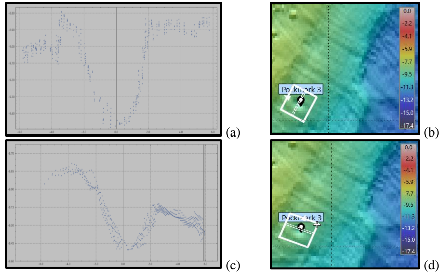
Fig. 11. Bathymetric profile of Pockmark 3 (Unit Pockmark), the largest surveyed depression. (a) Slice view along the pockmark formation, (b) Illustration of inspection area used for dimension analysis, (c) Slice view across the pockmark formation, (d) Illustration of inspection area used for dimension analysis
