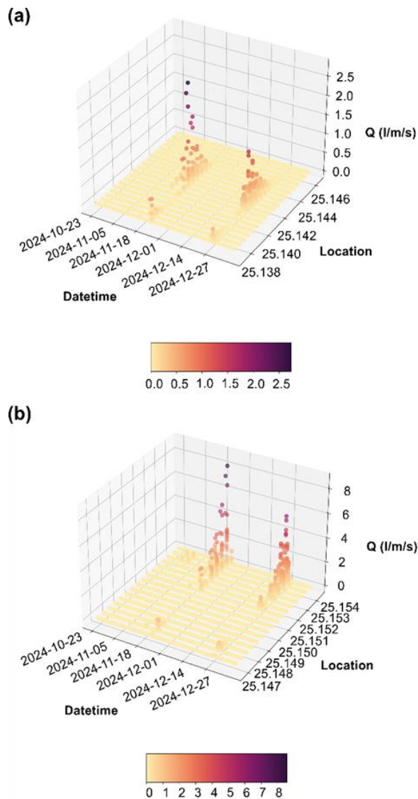
Fig. 10. The wave overtopping, Q \text{ (l/m/s)} , is estimated in the outside region of the pier. (a) Q time series estimated at the left side of the pier, and (b) at the right side of the pier at each grid point (Location, in °E)
