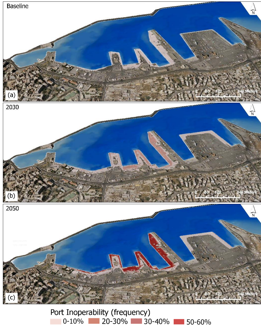
Fig. 7. Operability maps of the port of Heraklio for (a) Baseline period, (b) 2030 and (c) 2050
